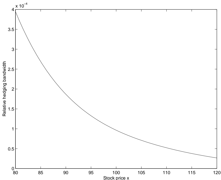
Figure 3: Relative hedging bandwidth \hat{\gamma}\sqrt{\varepsilon}\Upsilon(0.5, x)/\bar{\Delta}(0.5, x) for the parameter values given in Figure 2.
