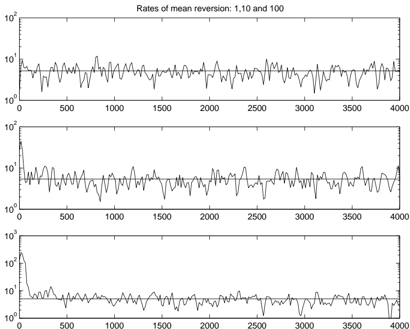
Figure 6: Spectrum of the logarithm of the square of a simulated normalized fluctuation process D_n , defined in (22), with rate of mean reversion \alpha = 1 in the top graph, \alpha = 10 in the middle one and \alpha = 100 in the bottom. The horizontal line is the mean plus 5%. The data simulates 120 trading days with 32 points per day and the window size of the FFT is 512 points (16 days).
