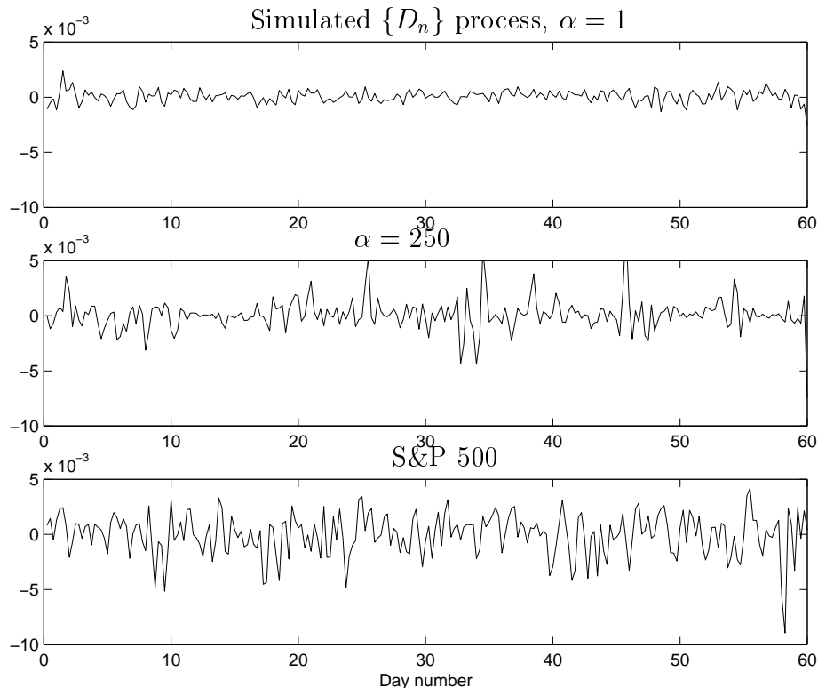
Figure 3: The top 2 figures show simulated paths of D_n , the de-meaned returns process defined in (22) with \alpha = 1 and \alpha = 250 , respectively. The other parameter values are: \bar{\sigma} = 0.04 , \nu = 1 , \rho = -0.1 . The simulations are done over 60 days with 1024 points per day. This time series is then decimated to 4 points per day, leaving 240 points, which is what is shown. The 3rd figure is the S&P 500's normalized fluctuation process from the first 60 trading days of 1994 decimated to 240 points total.
