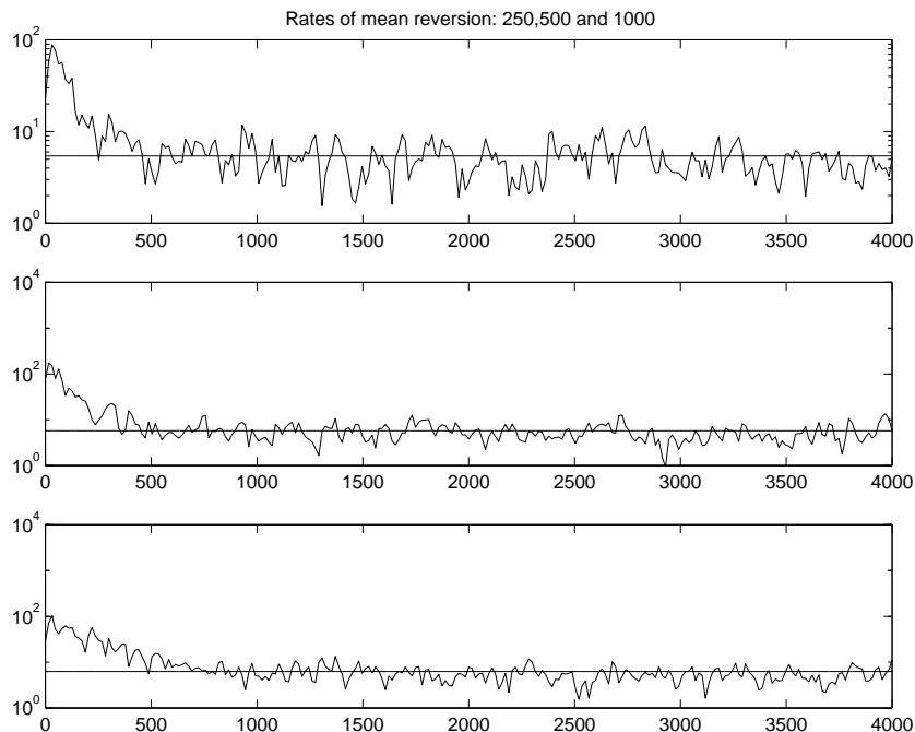
Figure 7: Spectrum of the logarithm of the square of a simulated normalized fluctuation process D_n , defined in (22). From top to bottom, the rates of mean-reversion are \alpha = 250, 500, 1000 . The data simulates 120 trading days with 32 points per day and the window size of the FFT is 512 points (16 days).
