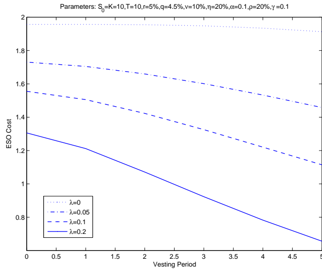
Figure 6: Effect of job termination risk: The ESO cost decreases significantly as the job termination risk rises. Furthermore, the cost decreases as vesting period lengthens due to the increasing likelihood of forfeiture.
