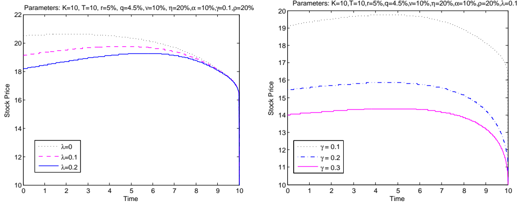
Figure 2: Effects of job termination risk and risk aversion: (Left) Higher job termination risk lowers the exercise boundary. (Right) As risk aversion \gamma increases, the employee's exercise boundary moves downward.
