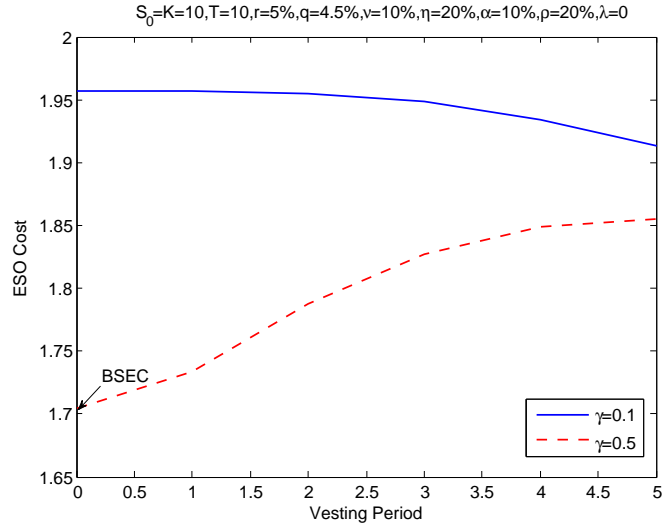
Figure 5: Effect of vesting: The marker “BSEC” represents the no-arbitrage price of a European call with the same strike and maturity as the ESO. In the absence of job termination risk, the cost of an ESO held by a very risk-averse employee increases (from close to BSEC) with respect to vesting. In the low risk aversion case, the cost decreases with vesting but stays above BSEC.
