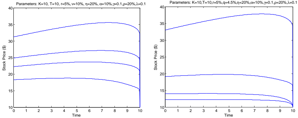
Figure 3: Effects of dividend rate and drift: (Left) The employee's exercise boundary exists even when the dividend rate is zero. It shifts downward as dividend rate, q , increases (from top to bottom, q = 0\% , 2\% , 3\% , 5\% ). (Right) The employee's exercise boundary is also monotone with respect to the stock's drift (from top to bottom, \nu = 15\% , 10\% , 5\% , 0\% ).
