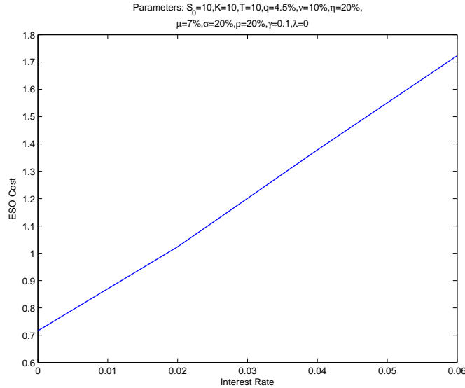
Figure 7: Effect of interest rate: As interest rate increases from 0% to 6%, the cost of the ESO doubles.
