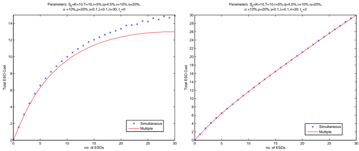
Figure 10: Effect of multiple exercises: (Left) When there is no vesting, the cost of ESOs with simultaneous exercise constraint dominates that with multiple exercise rights. (Right) However, when vesting is imposed, the difference in costs almost disappears.
