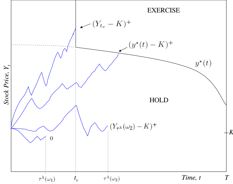
Figure 1: ESO payoff structure. The bottom path represents the scenario where the employee leaves the firm during the vesting period, resulting in forfeiture of the ESO. In the next path above, the employee is forced to exercise the ESO early due to job termination. The second from the top path hits the optimal exercise boundary y^*(t) after vesting, so the employee exercises the ESO there. The top one represents that the employee exercises the ESO immediately at the end of vesting.
