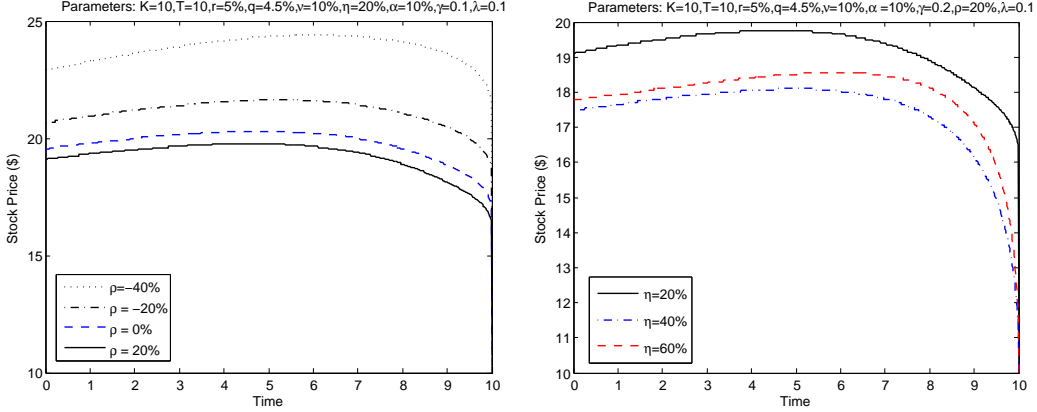
Figure 4: Effects of correlations and volatilities: (Left) When the market index (partial spanning asset) has a positive Sharpe ratio of 10%, the ESO holder's exercise boundary moves upward as the correlation becomes more negative. (Right) The employee's exercise boundary moves downward when stock volatility increases from 20% to 40%. When the volatility is raised to 60%, it moves upwards again. This shows that the employee's exercise boundary is not monotone with respect to the stock volatility.
