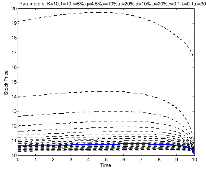
Figure 9: Multiple exercise boundaries: The dashed curves represent the exercise boundaries for an employee with 30 ESOs with multiple exercise rights. The bottom one corresponds to the first option exercised, and the top one corresponds to the last option exercised. When the employee is granted 30 ESOs with simultaneous exercise constraint, his exercise boundary (solid line) lies somewhere in the middle.
