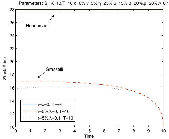
Figure 8: Comparing exercise boundaries: The model by Henderson (2006) gives a high flat exercise boundary. Grasselli (2005) corresponds to the middle boundary. The bottom boundary from our model accounts for the presence of job termination risk. The parameter values are chosen so that the exercise boundary by Henderson (2006) is finite.
